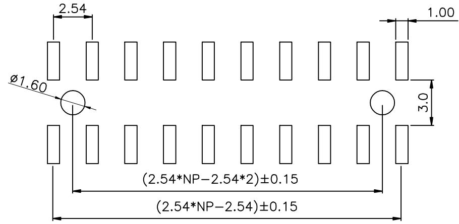
PCB LAYOUT
