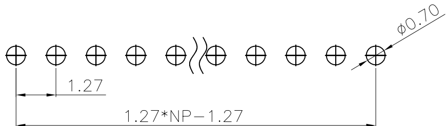
PCB LAYOUT
